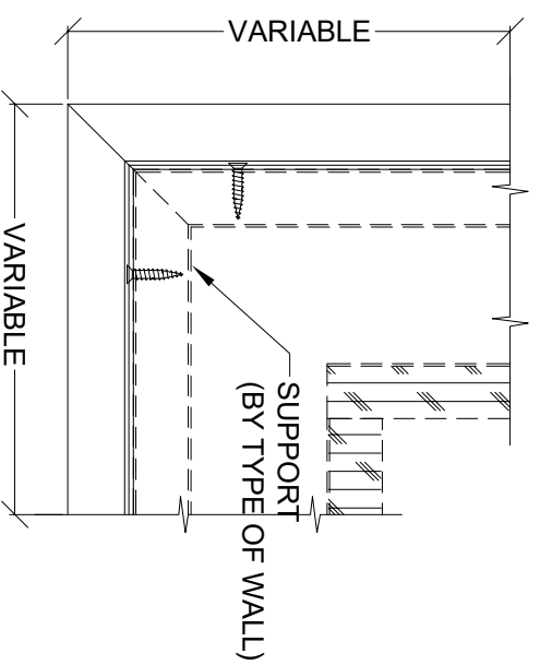
OUTSIDE CORNER DETAIL (PLAN VIEW)
